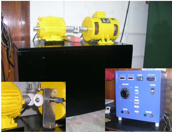
A Sophisticated Gear Test Rig Designed to Evaluate Novel Gear Designs.
