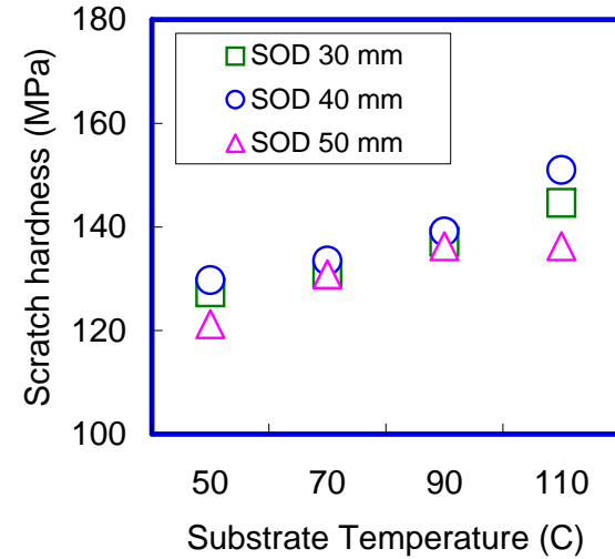
Scratch hardness different coated samples
