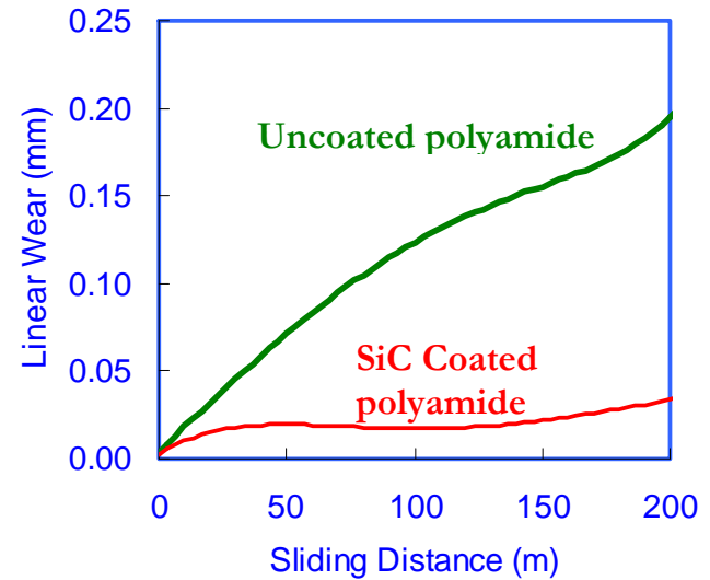
Abrasive wear of coated and uncoated polyamides
