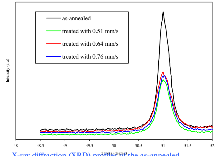
X-ray diffraction (XRD) profiles of the as-annealed and treated samples showing nanostructure formed
